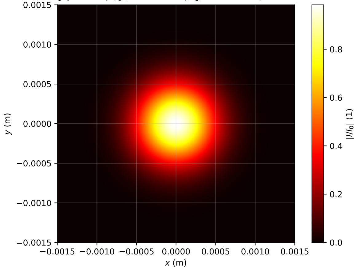
Intensity profile I(x, y, z = 0.318m)/I_0 , P_{in}=0.1P_{cr} , artificial time
